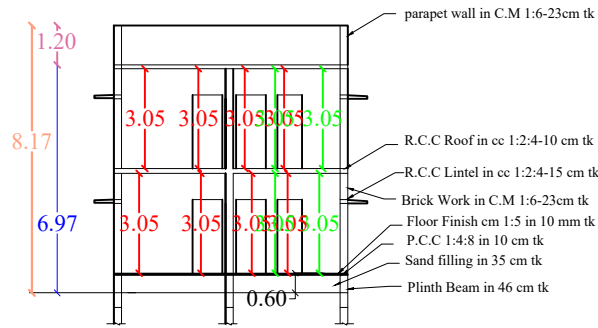
SECTION ON "AR"
