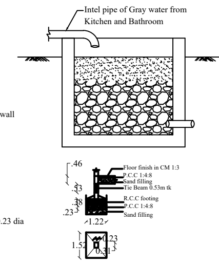
GREY WATER RECYCLING CHAMBER:-
