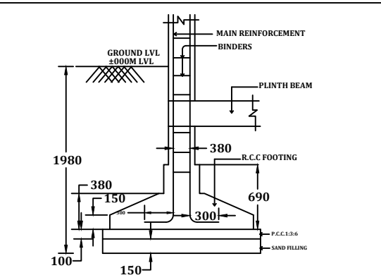
R.C.C COLUMN FOUNDATION
