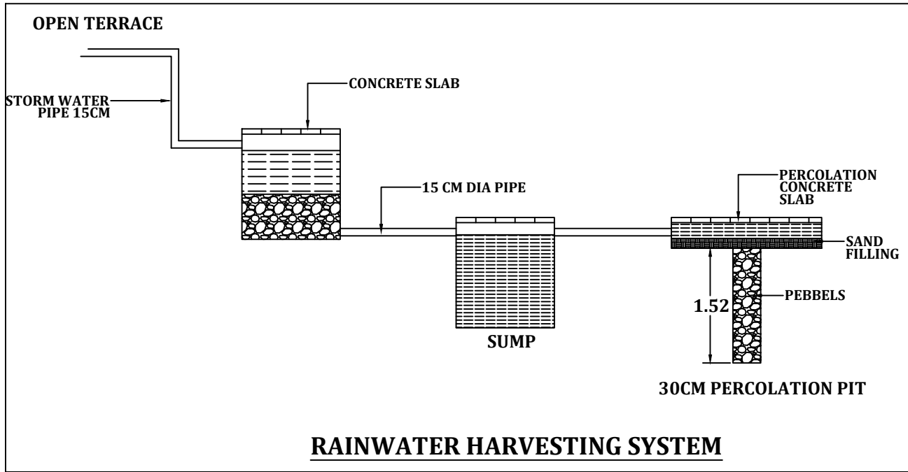
RAINWATER HARVESTING SYSTEM
