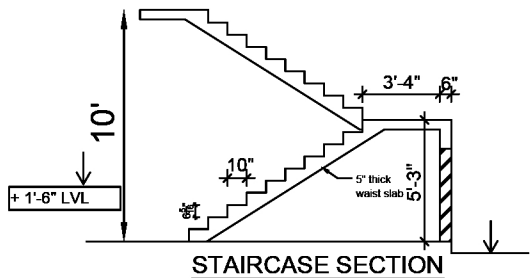
STAIRCASE SECTION
