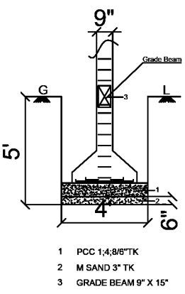
Foundation Details 4' x 4' x 5'
