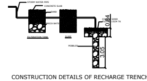
CONSTRUCTION DETAILS OF RECHARGE TRENCH
