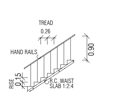
STAIRCASE DETAILS
