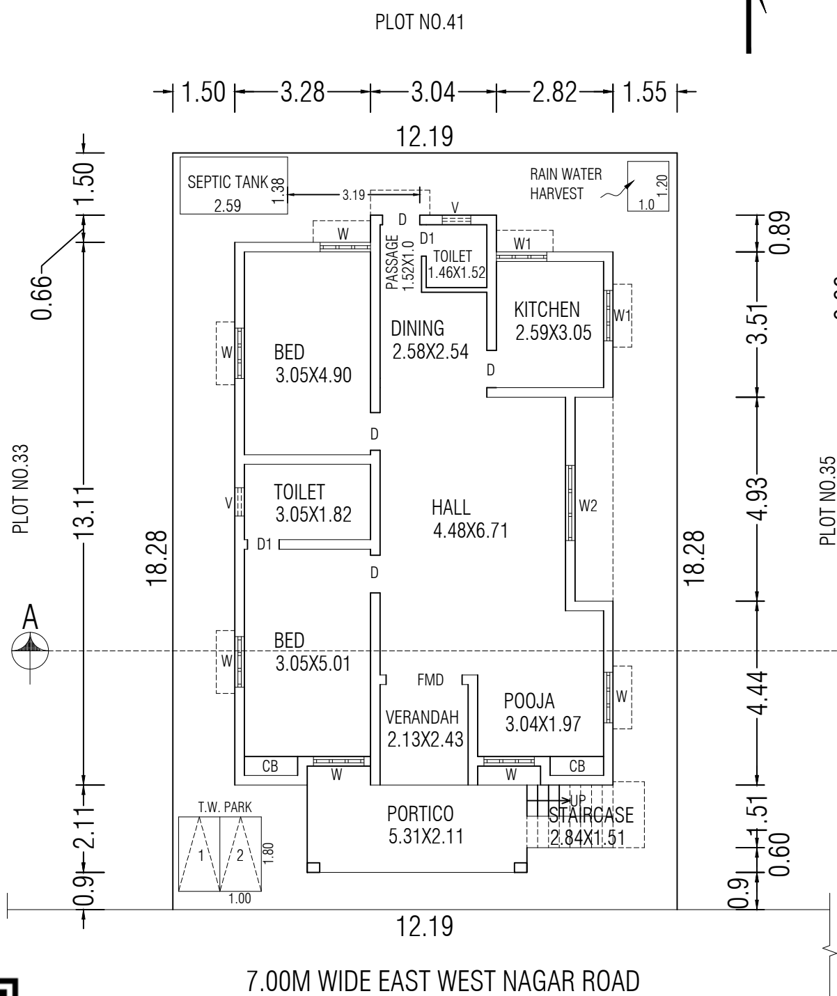
SITE CUM EXISTING GROUND FLOOR PLAN
