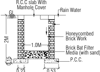
DETAILS OF RAIN WATER COLLECTION PIT
