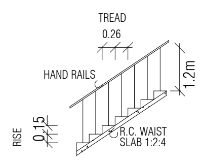
STAIRCASE DETAILS
