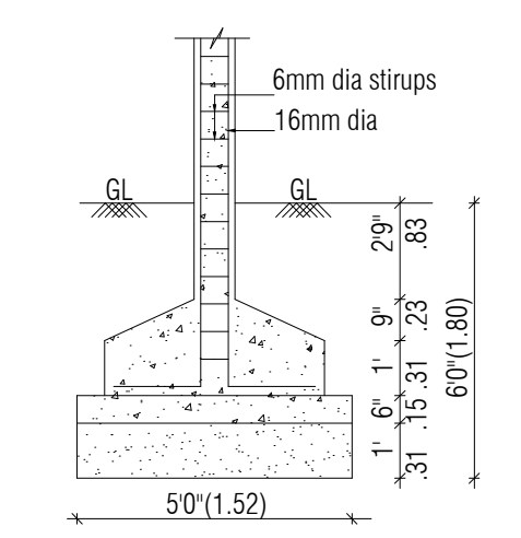
FOUNDATION DETAIL
