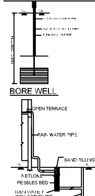
RAIN WATER
