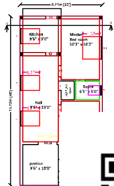
GROUND FL
