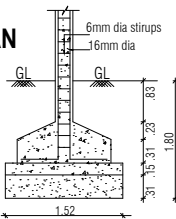
FOUNDATION DETAIL
