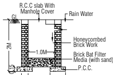
DETAILS OF RAIN WATER COLLECTION PIT
