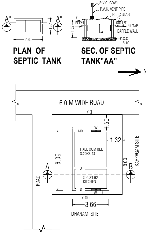
SITE CUM GROUND FLOOR PLAN
