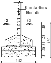
FOUNDATION DETAIL
