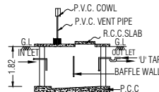
SEC. OF SEPTIC TANK "AA"
