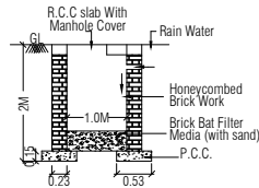
DETAILS OF RAIN WATER COLLECTION PIT
