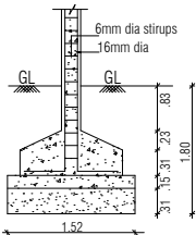
FOUNDATION DETAIL
