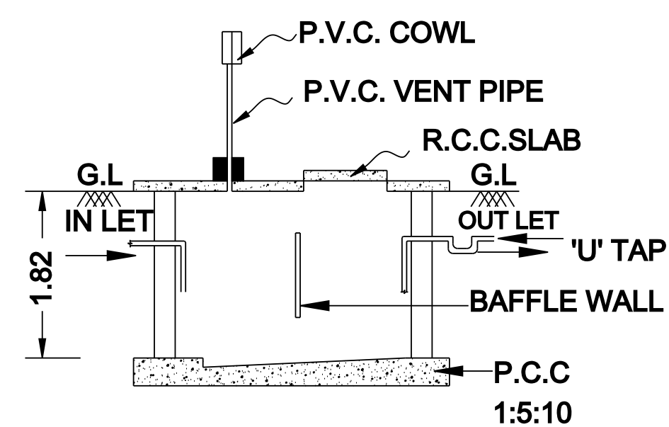
SEC. OF SEPTIC TANK"AA"
