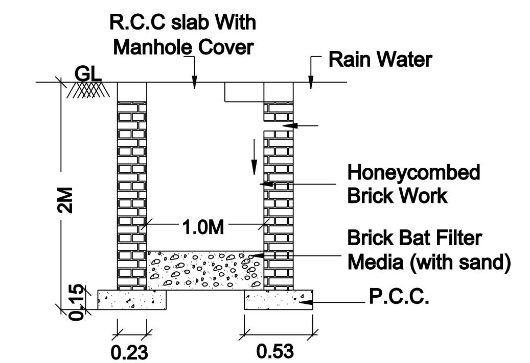
DETAILS OF RAIN WATER COLLECTION PIT
