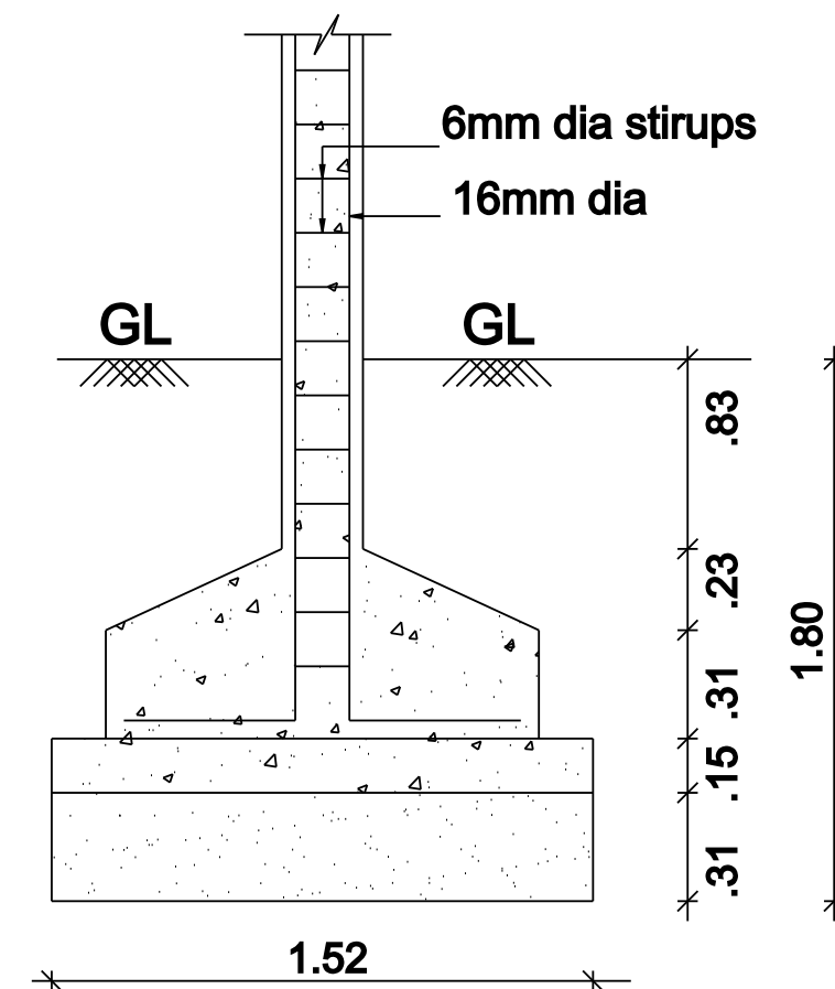
FOUNDATION DETAIL
