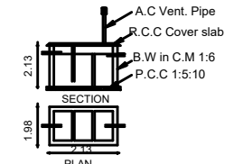
SEPTICTANK DETAILS
