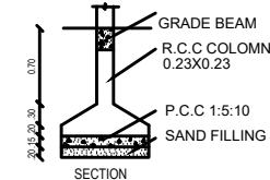
FOUNDATION DETAILS
