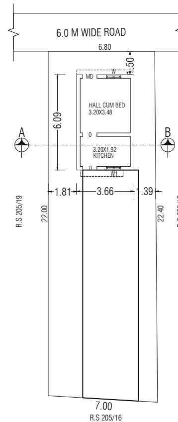
SITE CUM GROUND FLOOR PLAN
