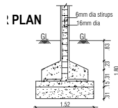
FOUNDATION DETAIL
