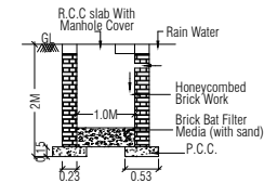
DETAILS OF RAIN WATER COLLECTION PIT
