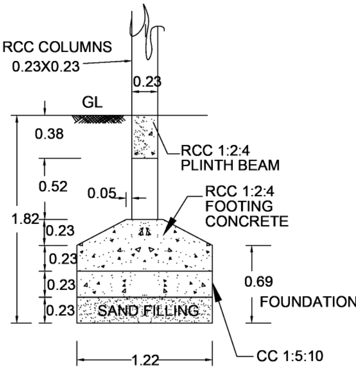
FOUNDATION DETAILS
