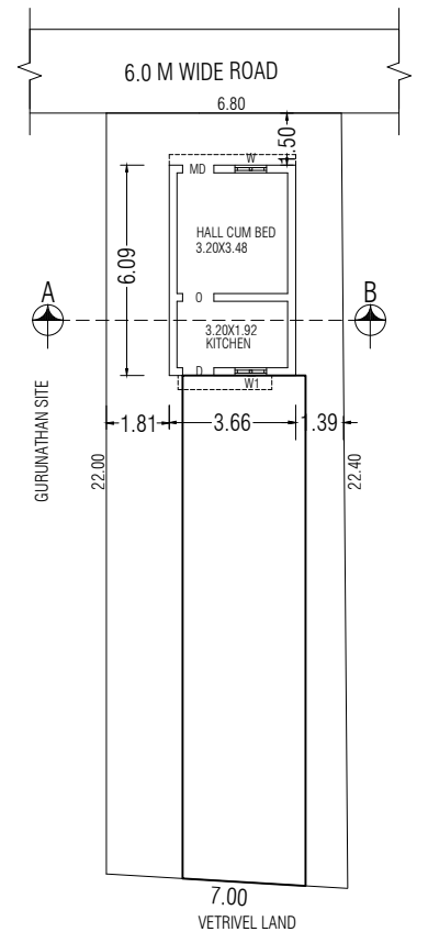
SITE CUM GROUND FLOOR PLAN
