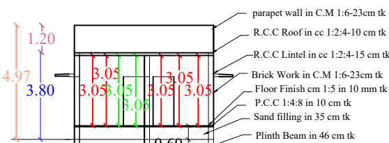
SECTION ON "AR"
