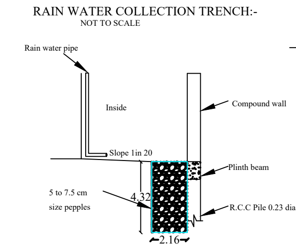
RAIN WATER COLLECTION TRENCH:- NOT TO SCALE
