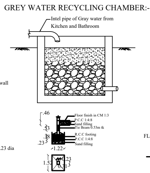
GREY WATER RECYCLING CHAMBER:-
