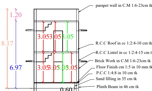
SECTION ON "AR"
