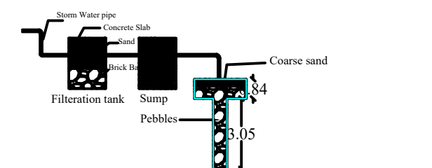
CONSTRUCTION DETAILS OF RECHARGE TRENCH
