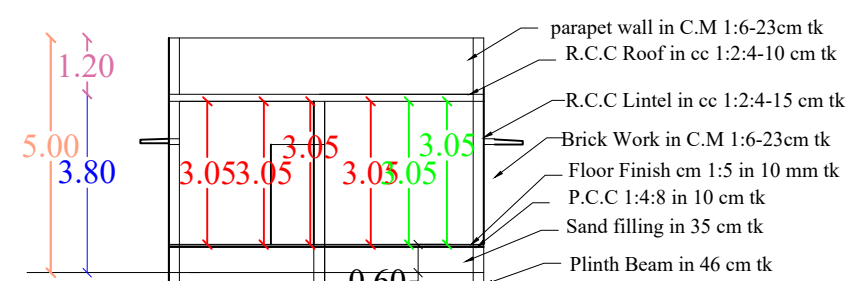
SECTION ON "AR"
