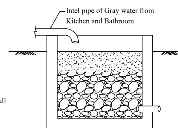
GREY WATER RECYCLING CHAMBER:-
