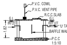
SEC. OF SEPTIC TANK "AA"
