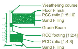
Foundation Details
