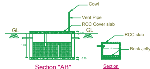
Section "AB"
