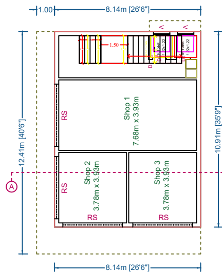
Ground Floor plan=0 Ground Floor Plan
