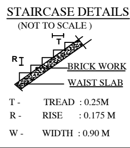
STAIRCASE DETAILS
