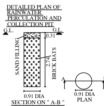
DETAILED PLAN OF RAINWATER PERCOLATION AND COLLECTION
