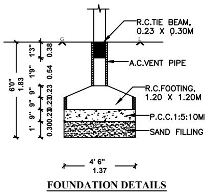
FOUNDATION DETAILS
