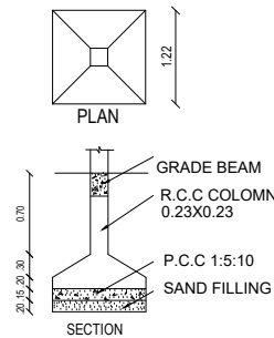
FOUNDATION DETAILS
