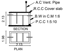
SEPTICTANK DETAILS
