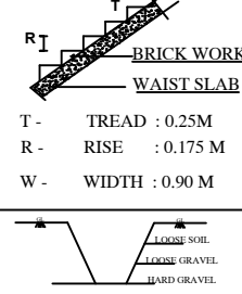
STAIRCASE DETAILS (NOT TO SCALE)
