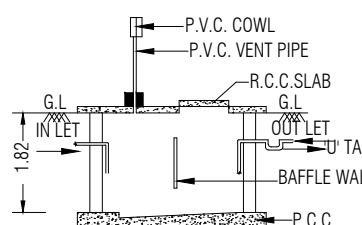
SEC. OF SEPTIC TANK"AA"
