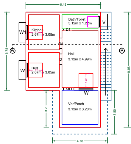
GROUND_FLOOR_PLAN=0
