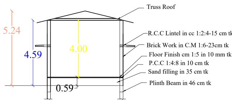
SECTION ON "AR"
