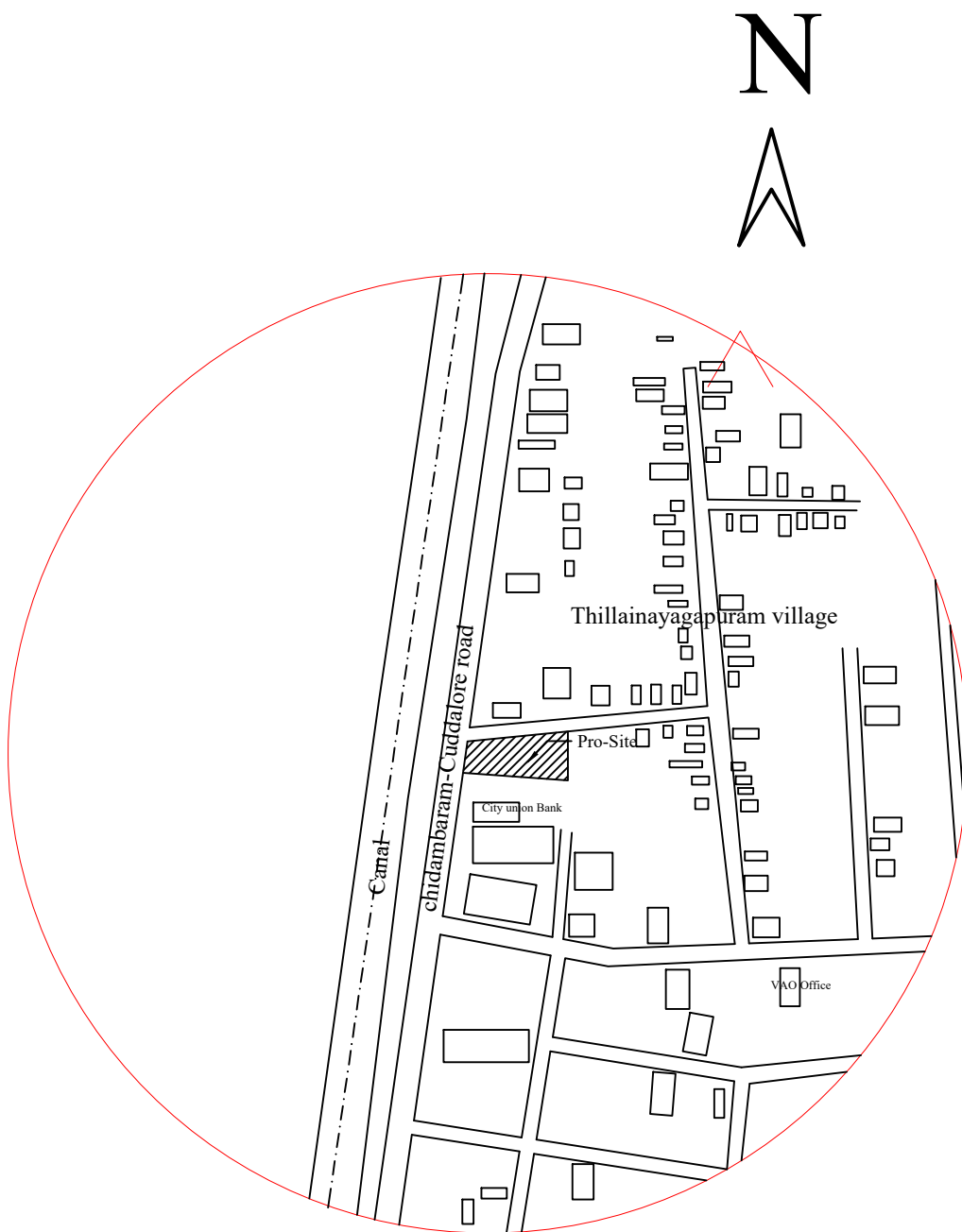
TOPO PLAN(300M R )scale 1:5000
