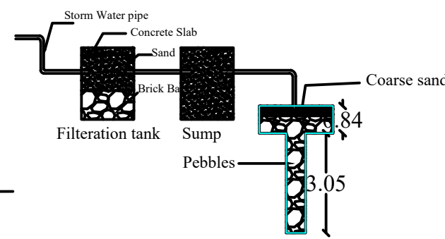
CONSTRUCTION DETAILS OF RECHARGE TRENCH
