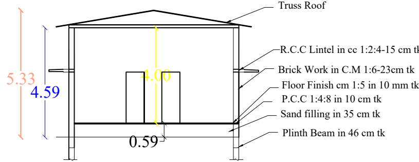
SECTION ON "AR"
