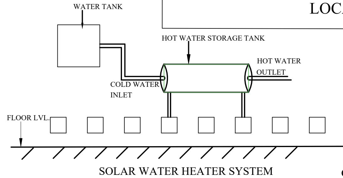
SOLAR WATER HEATER SYSTEM
