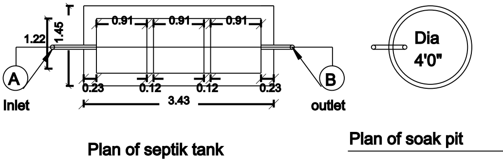
Plan of septic tank
