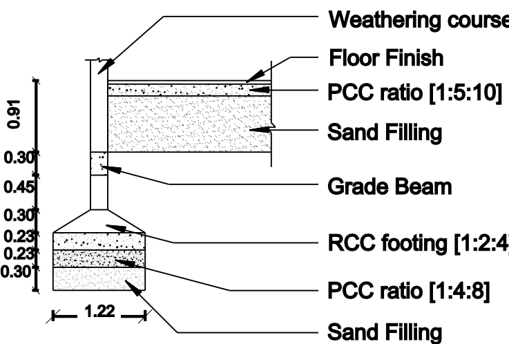
Foundation Details
