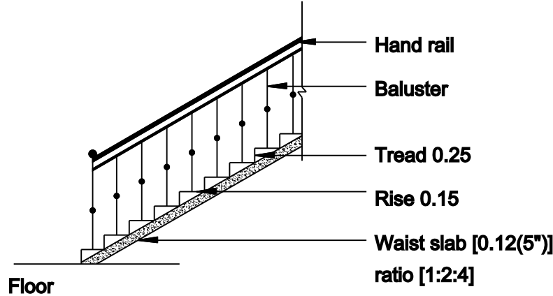
Staircase Details
