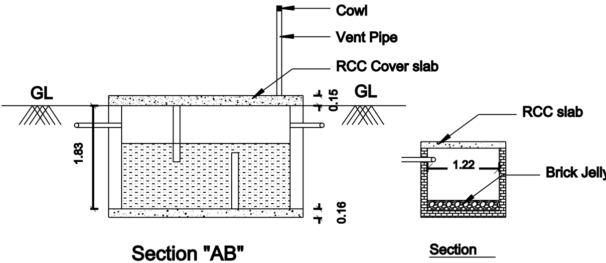
Section "AB"
