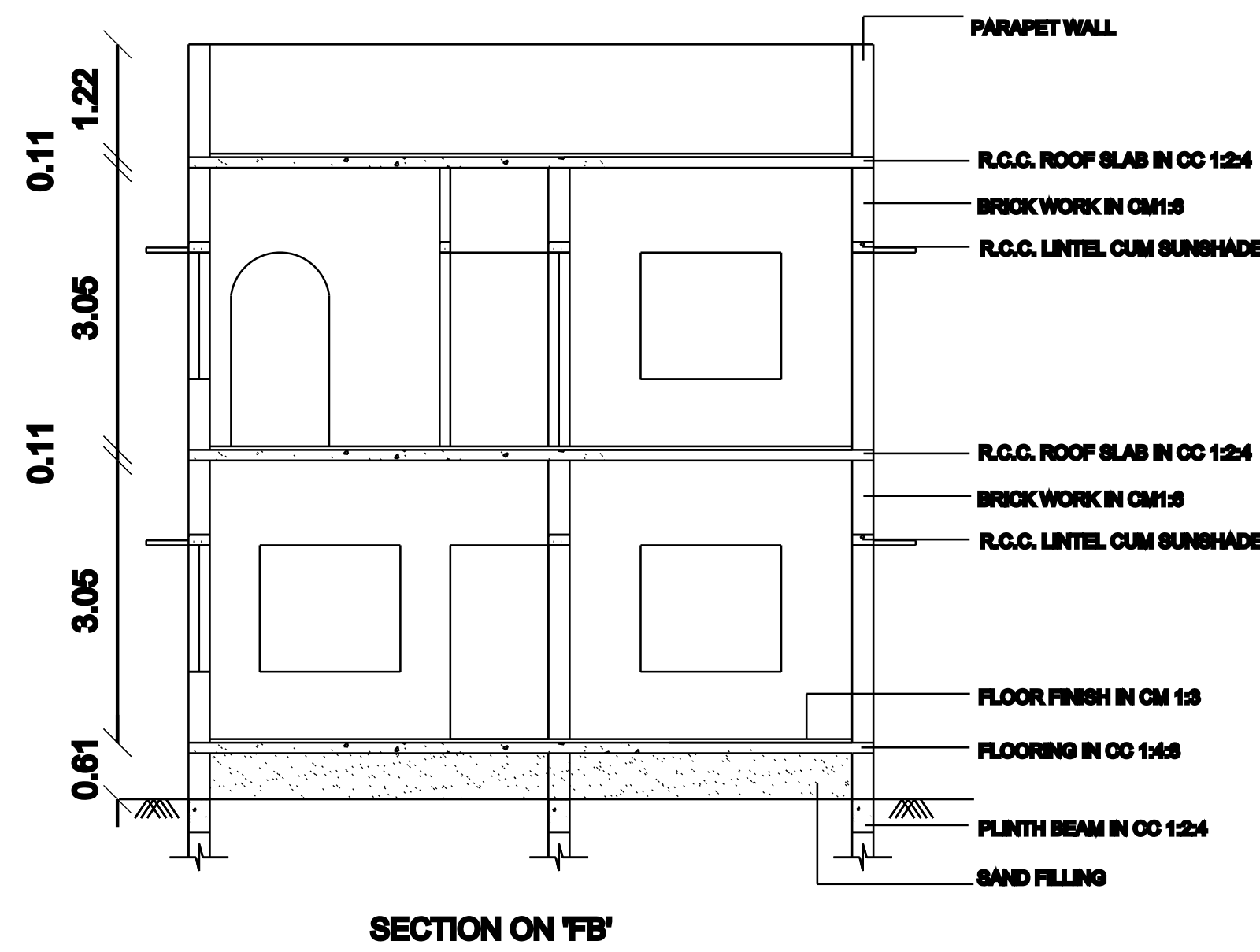
SECTION ON 'FB'
