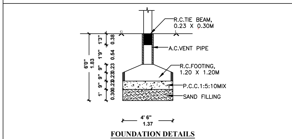
FOUNDATION DETAILS
