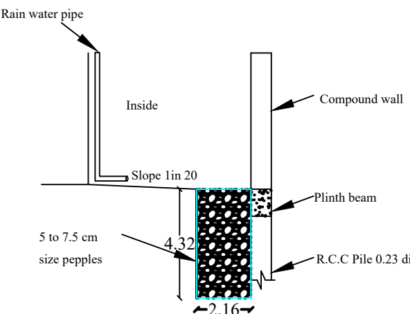
RAIN WATER COLLECTION TRENCH:- NOT TO SCALE
