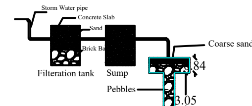
CONSTRUCTION DETAILS OF RECHARGE TRENCH
