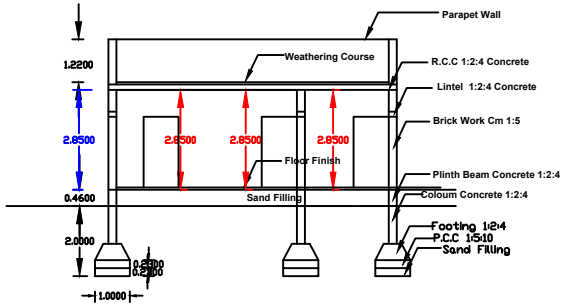
Section Section - AA
