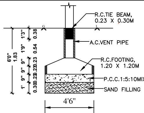
FOUNDATION DETAILS
