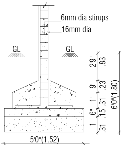
FOUNDATION DETAIL
