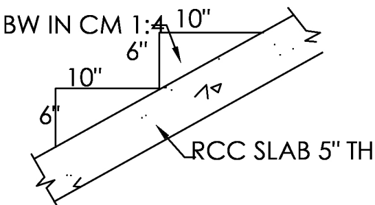
STAIR DETAIL
