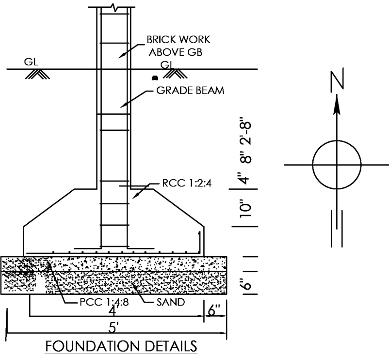
FOUNDATION DETAILS
