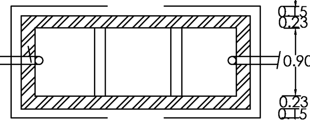
PLAN AND SECTION OF SEPTIC TANK
