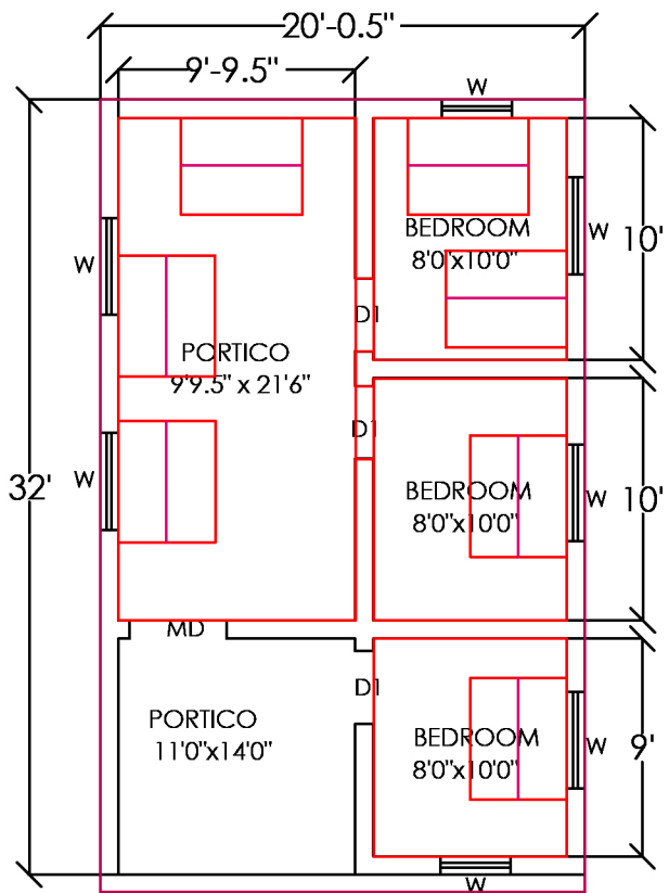
GROOUND FLOOR PLAN
