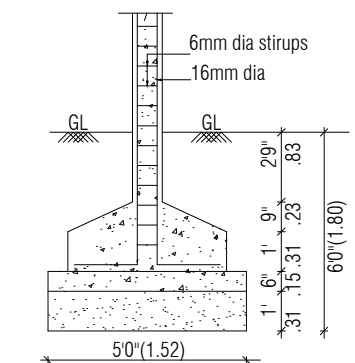
COLUMN FOUNDATION DETAIL
