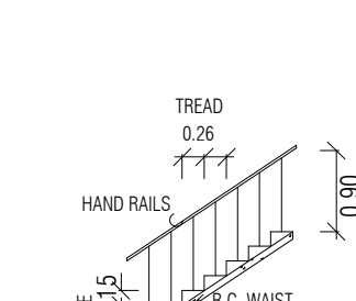
STAIRCASE DETAILS
