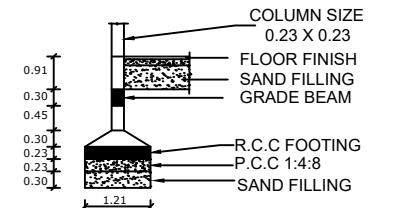
FOUNDATION DETAILS SCALE 1:500
