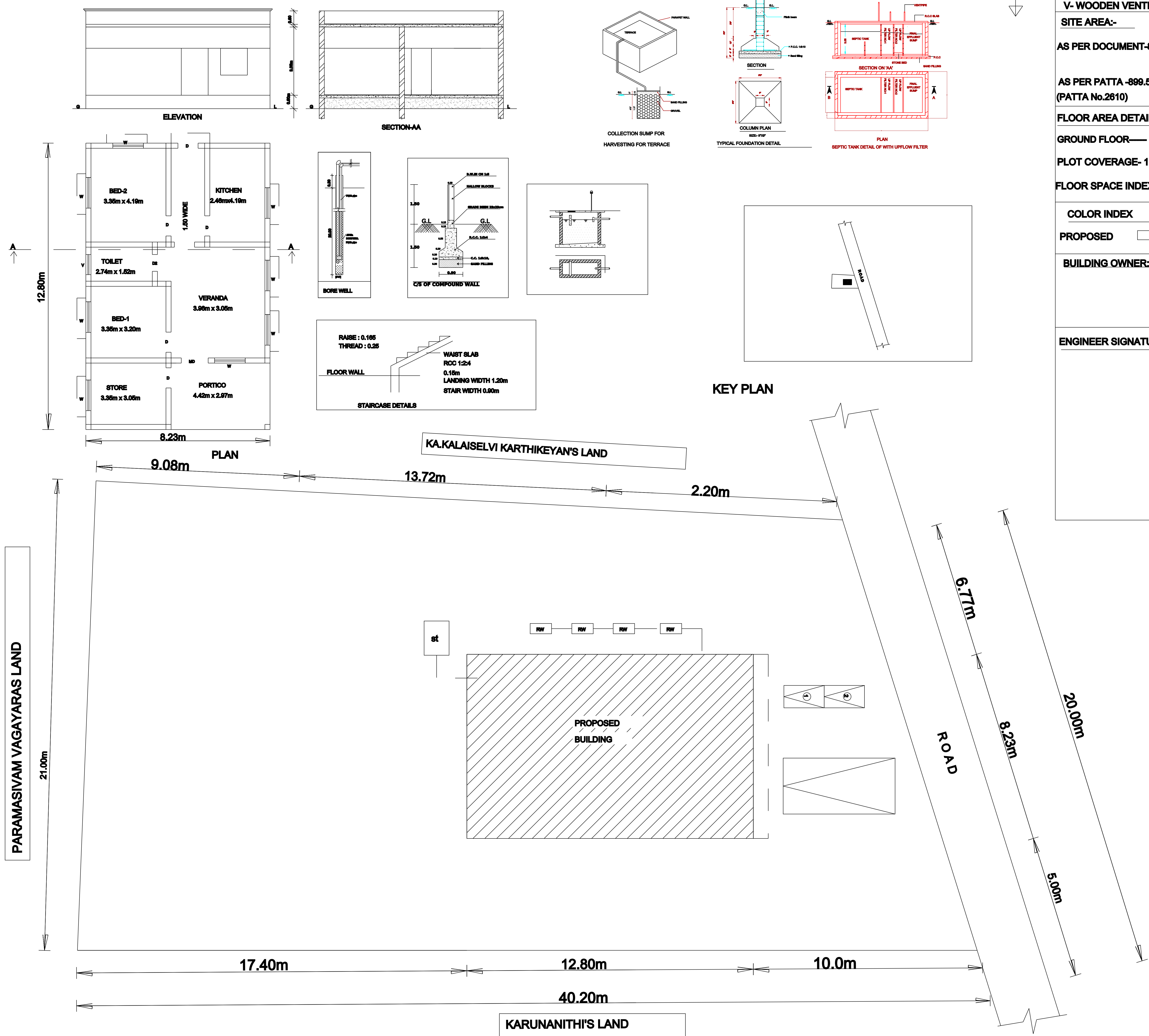
SITE PLAN
