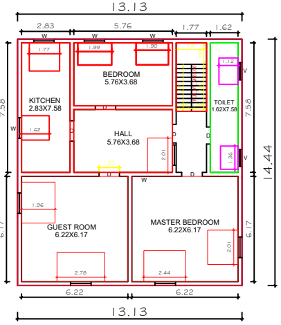
PRO. FIRST FLOOR HOUSE PLAN
