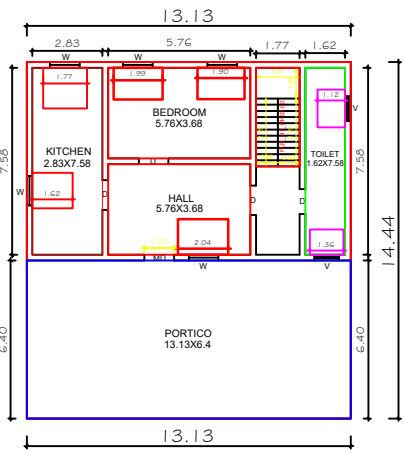
PRO. GROUND FLOOR HOUSE PLAN
