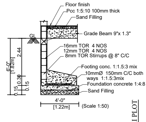
FOUNDATION DETAILS
