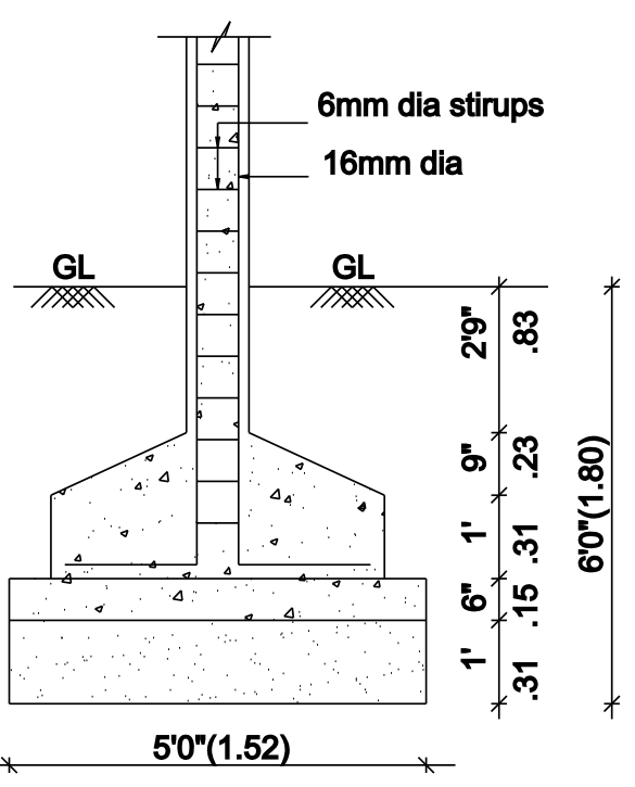
FOUNDATION DETAIL
