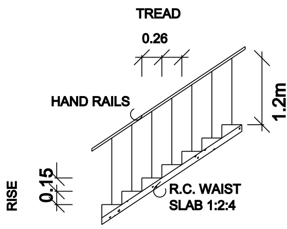
STAIRCASE DETAILS SCALE (1:50)
