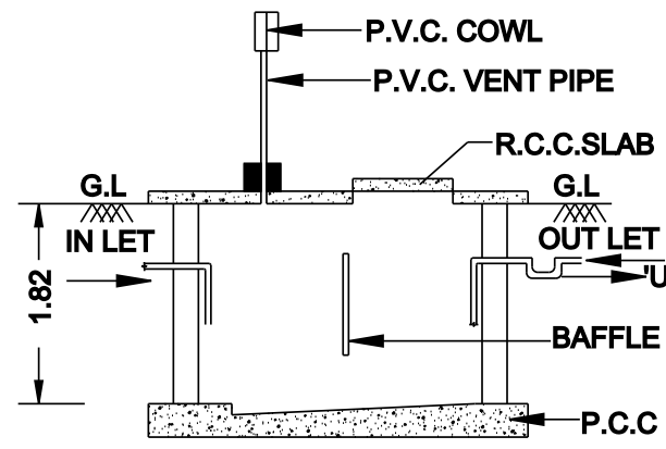
SEC. OF SEPTIC TANK"AA"
