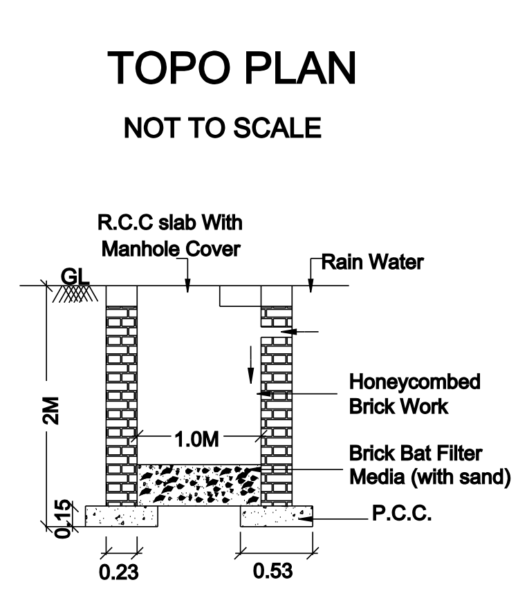
DETAILS OF RAIN WATER COLLECTION PIT
