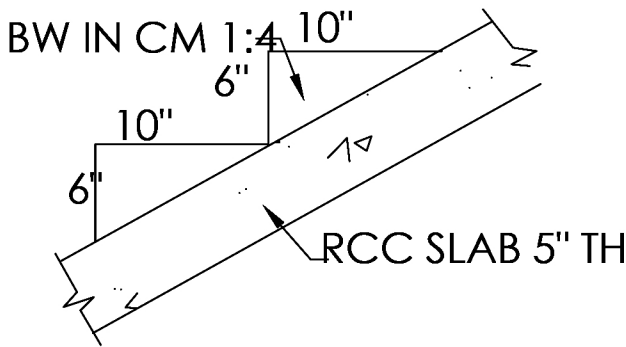
STAIR DETAIL
