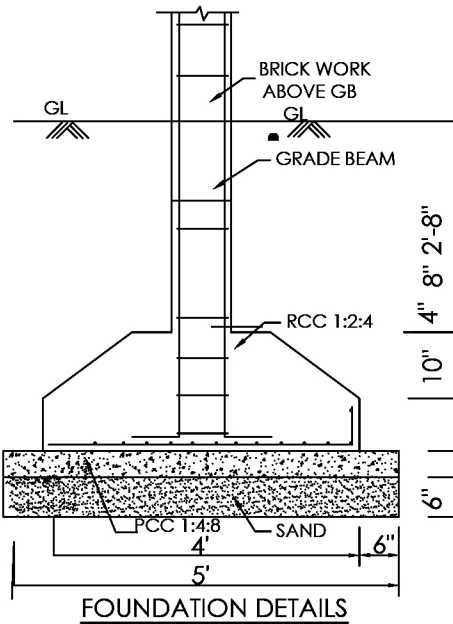
FOUNDATION DETAILS
