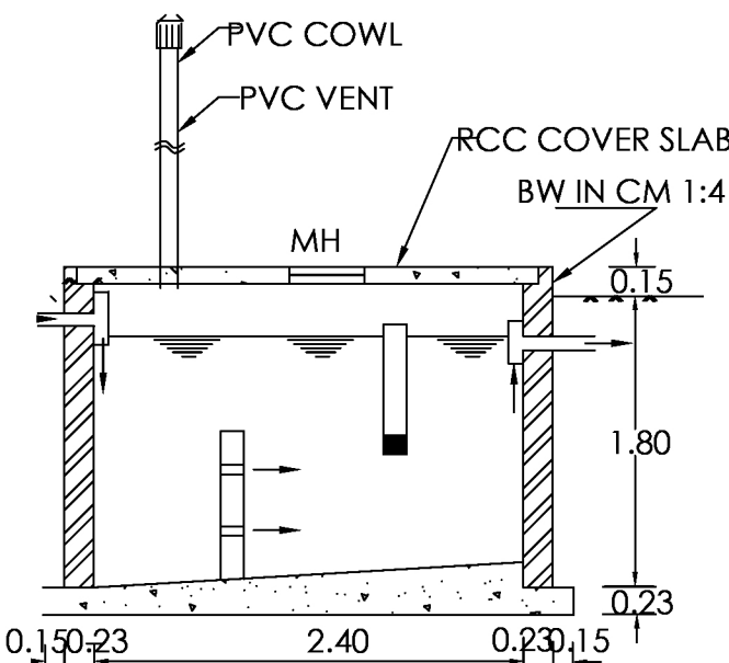
PLAN AND SECTION OF SEPTIC TANK
