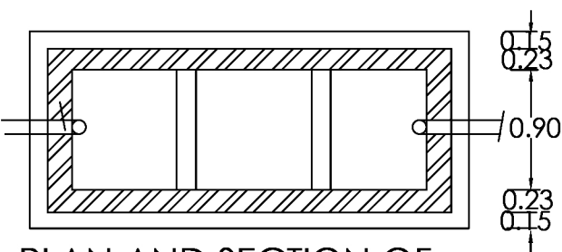
PLAN AND SECTION OF SEPTIC TANK
