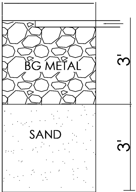
RAIN WATER
