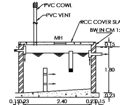
PLAN AND SECTION OF SEPTIC TANK
