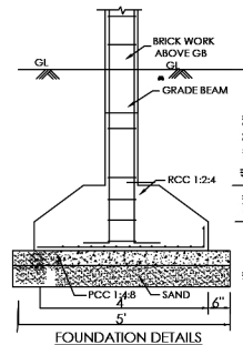
FOUNDATION DETAILS
