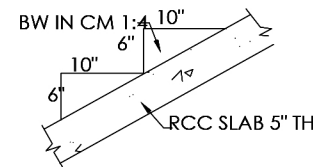
STAIR DETAIL
