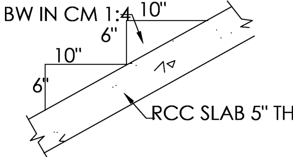
STAIR DETAIL
