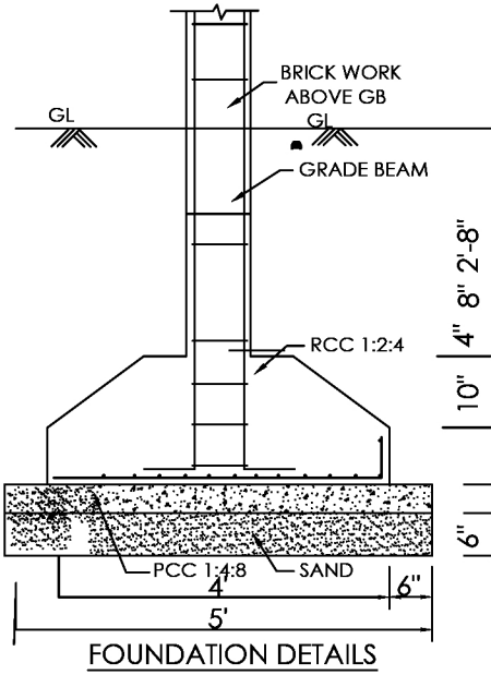
FOUNDATION DETAILS
