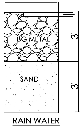
RAIN WATER
