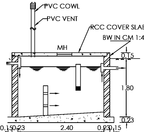
PLAN AND SECTION OF SEPTIC TANK
