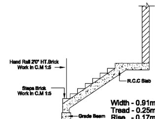
STAIR CASE DETAILS (Scale :- 1:100)
