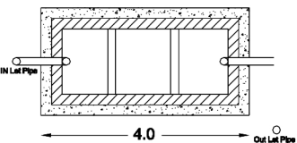
PLAN (Scale :- 1:100)
