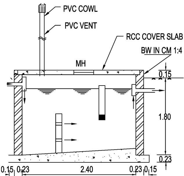
PLAN AND SECTION OF SEPTIC TANK
