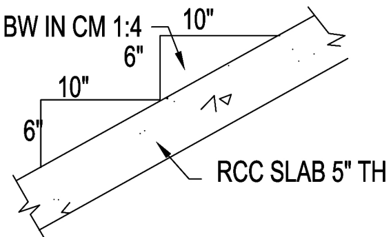
STAIR DETAIL
