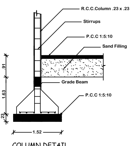
COLUMN DETAIL
