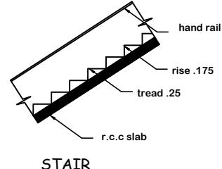
STAIR
