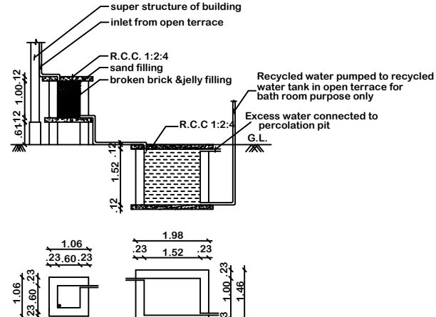
Sump and Filter Bed
