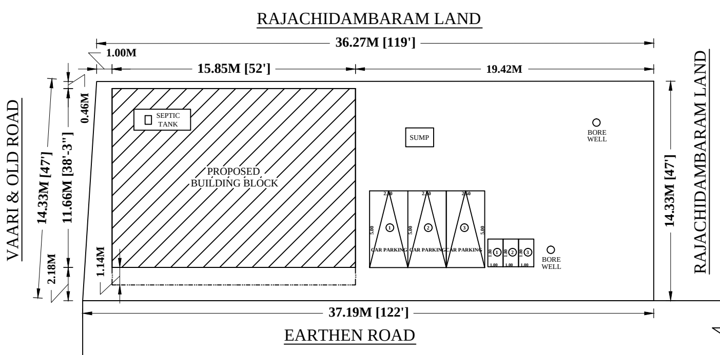
SITE PLAN SCALE IN 1:200
