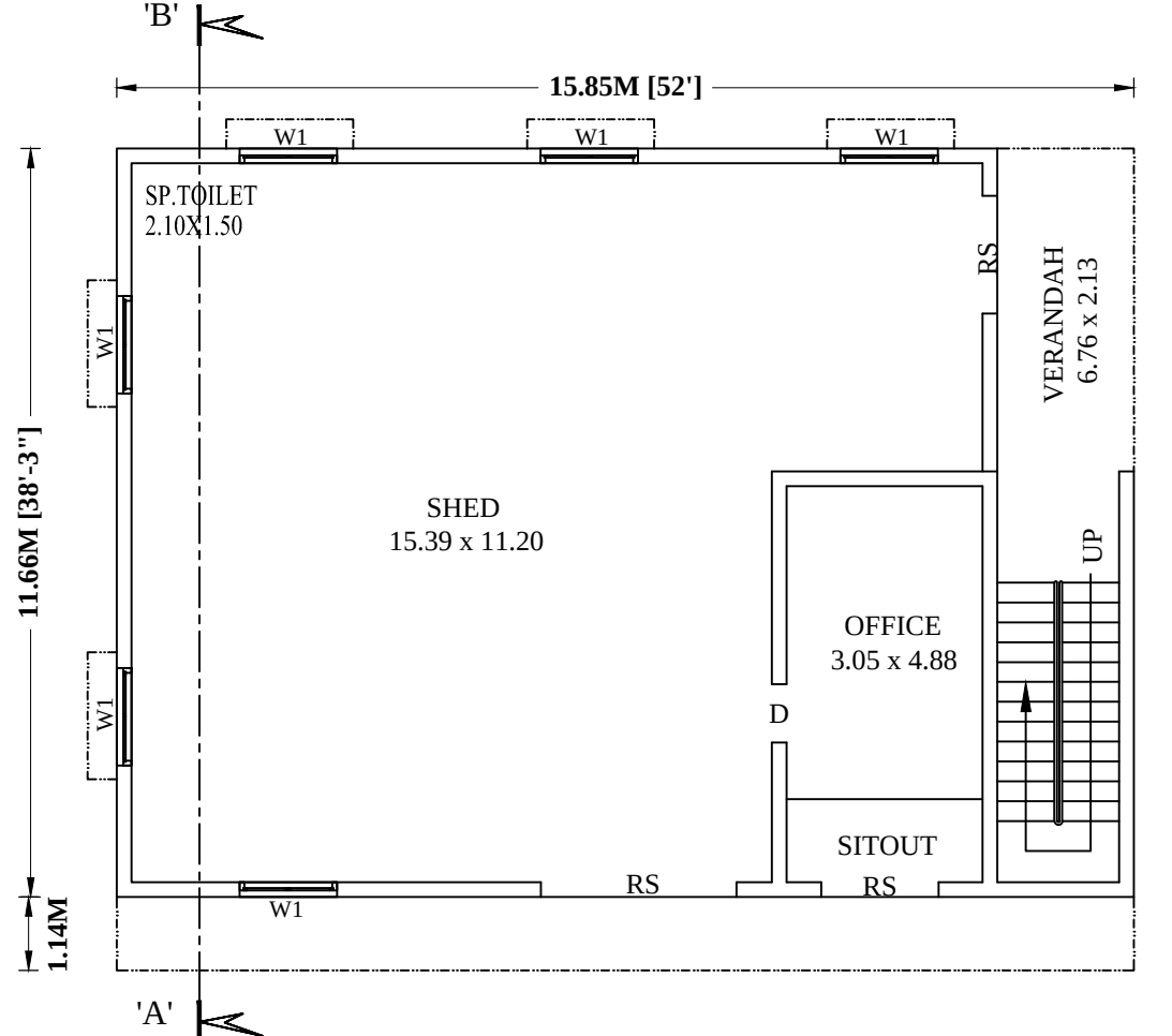
REVISED GROUND FLOOR PLAN
