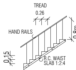
STAIRCASE DETAILS
