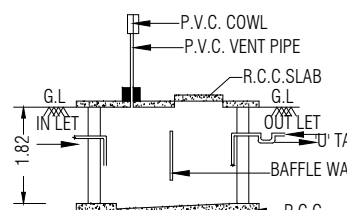
SEC. OF SEPTIC TANK"AA"
