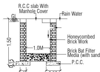
DETAILS OF RAIN WATER COLLECTION PIT SCALE:- 1"=4'0"
