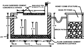
SECTION X-X
