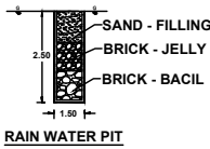
RAIN WATER PIT
