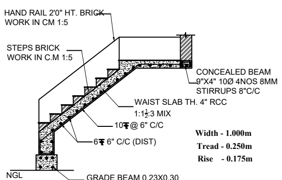
STAIRCASE DETAILS
