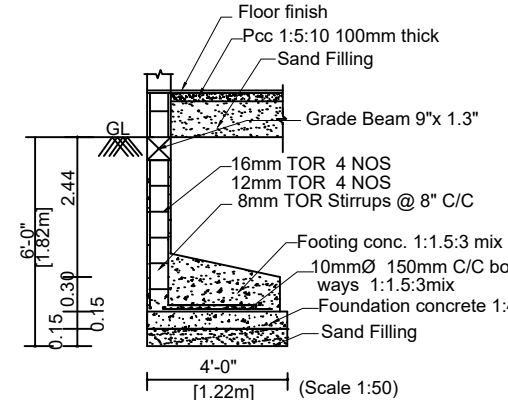
FOUNDATION DETAILS
